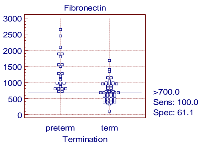
Figure 1. Optimal cutoff values, sensitivity and specificity obtained from ROC Curve analysis
