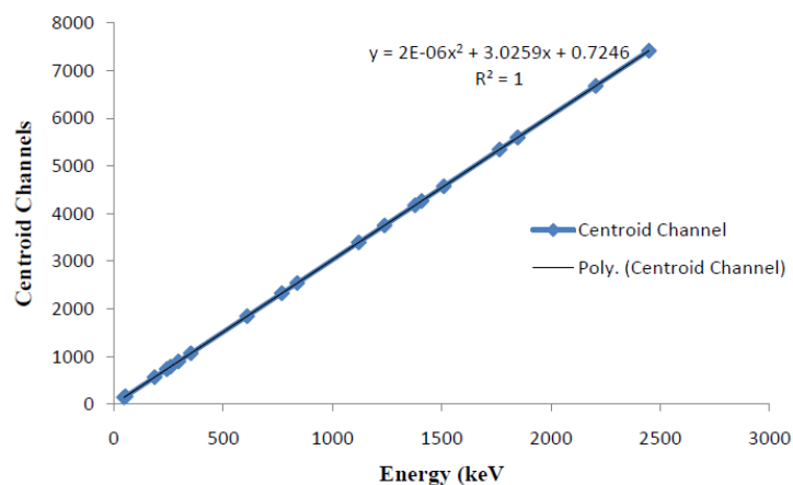
Figure2. Channels versus energy calibration
