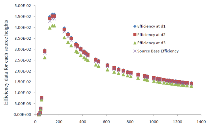
Figure3. Efficiency curve at d_1 , d_2 , d_3 and the mixed source base standard
